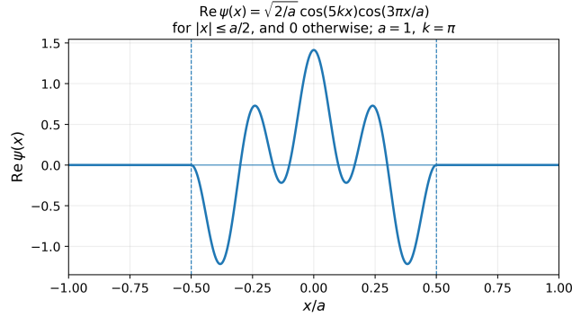
Figure 3.2: Plot of the real part of \psi(x) , for parameters a = 1 and k = \pi . Image generated by ChatGPT 5.6 Luna.
